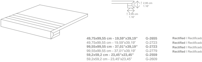
Step Type Gradone 1cm | Angular Type Gradone 1cm
