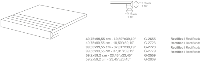
Step Type L 1cm | Angular Type L 1cm
