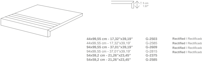
Step Type L 2cm | Angular Type L 2cm
