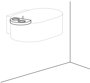
MENSOLA SEMICERCHIO IN CERAMICA / LEGNO IROKO Semicircular shelf ceramic / Iroko wood cm 28 x 18 x 3 h
