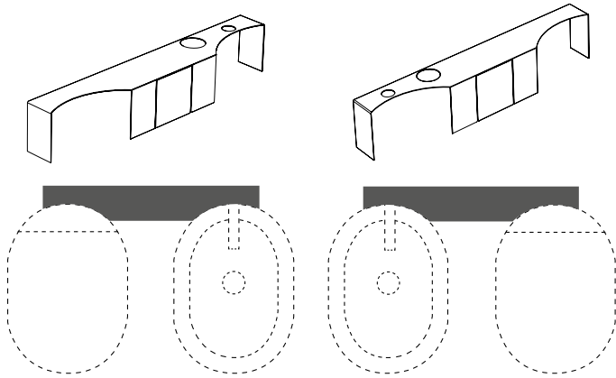
ACCESSORIO INTEGRATO WC E BIDET TERRA ITACA, CON FORO RUBINETTO, DISPENSER E PORTAROTOLO, DX/SX Integrated fitting for Itaca floor-standing WC and bidet, with tap hole, dispenser and toilet roll holder, right / left version cm 74 x 12 x 13 h
